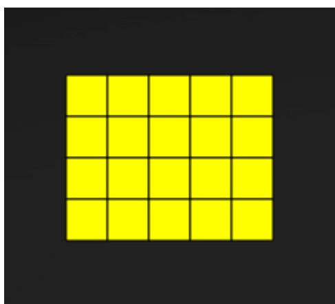
Figure 31 Example of a rectangle split into squares
